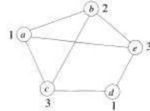
Figure 7.11 An example graph and its coloring
