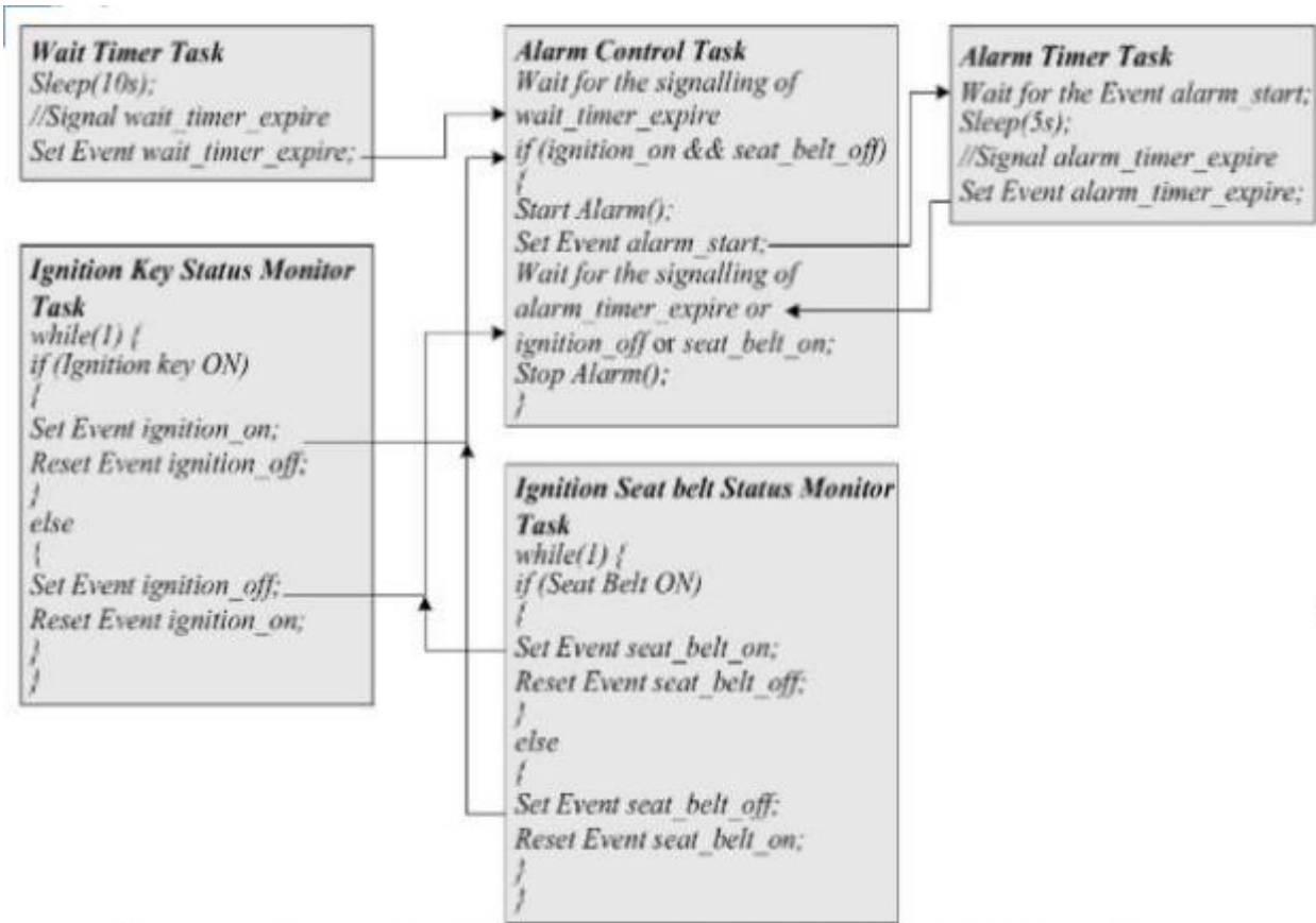
Concurrent processing Program model for "Seat Belt Warning" System
